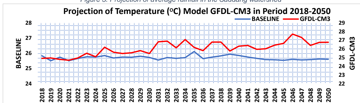
Figure 6. Projection of average temperature in a period of 2018-2050
