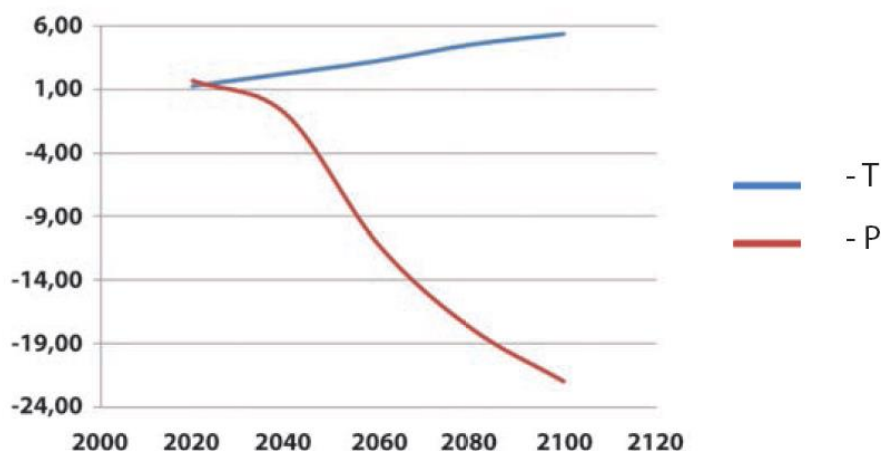
Fig. 4: Deviation from the normal average air temperature T ( 0 C) and precipitation P (mm) for Turkmenistan on averaged scenarios A1FI and B1, TNC
