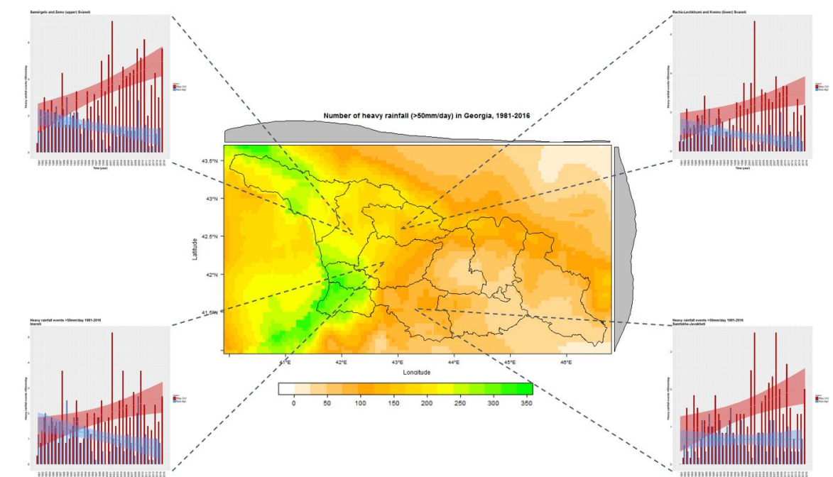
Figure 5 Number of heavy rainfall (>50mm/day) in Georgia 1981-2016. 6
