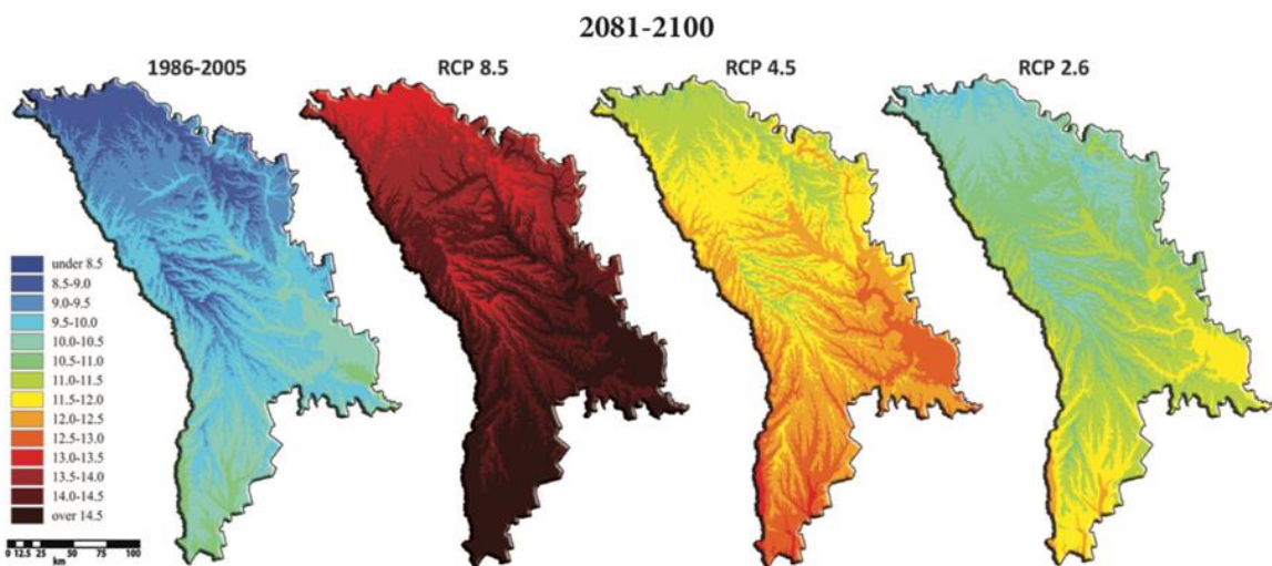
Figure 14 Projected CMIP5 GCMs Mean Annual Air Temperature °C 2081-2100
