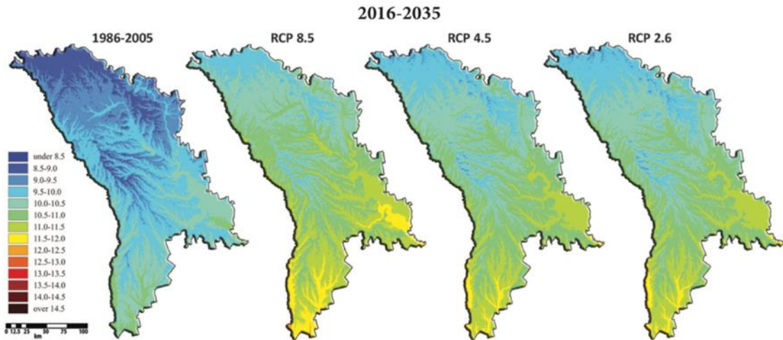
Figure 12 Projected CMIP5 GCMs Mean Annual Air Temperature °C 2016-2035
