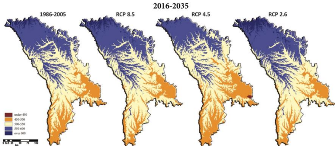
Figure 15 Projected CMIP5 21 GCMs Annual Precipitation, (mm) 2016-2035
