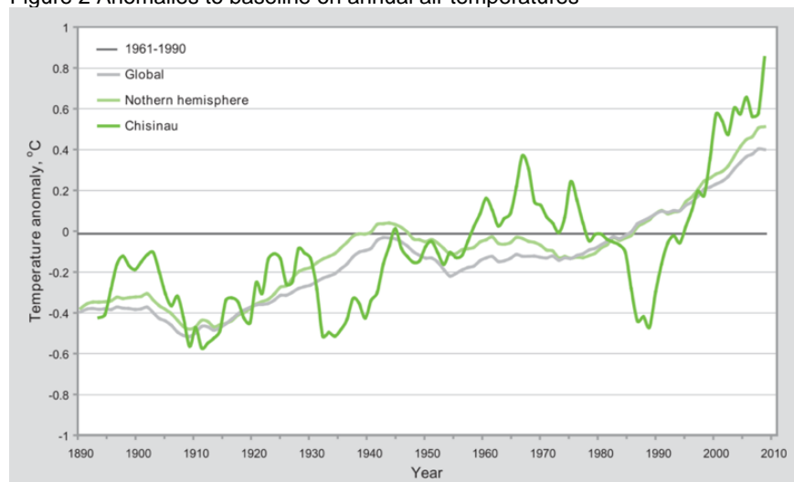
Figure 2 Anomalies to baseline on annual air temperatures 21,22
