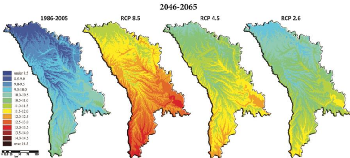
Figure 13 Projected CMIP5 GCMs Mean Annual Air Temperature °C 2046-2065
