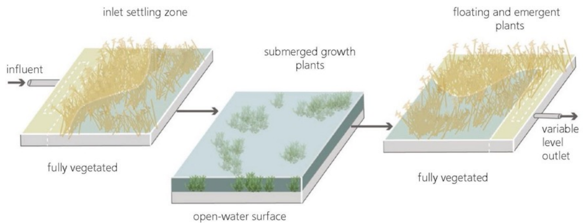
Figure 22: Schematic detail drawings of the proposed Bar Elias Constructed Wetland
