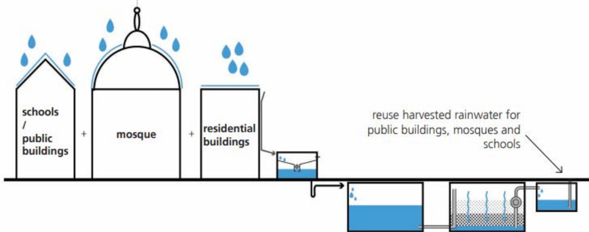
Figure 28: Schematic detailed drawing of rainwater harvesting systems proposed for schools/mosques/municipal buildings/residential buildings in Jordan
