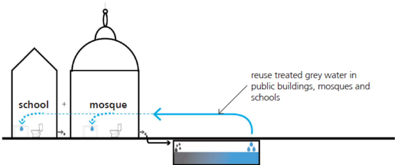
Figure 29: Greywater treatment and reuse: schematic detail section for greywater treatment and reuse system in schools and mosques
