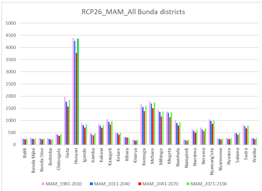
Figure 6b: Spatial historical and projected rainfall behavior in the project site for the longer rains' (March-April-May) for the period covering 1981-2100, under RPC 2.6 scenario.
