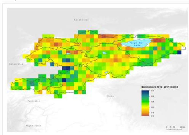
Figure 11 Average soil moisture during the current decade (2010-2017).
