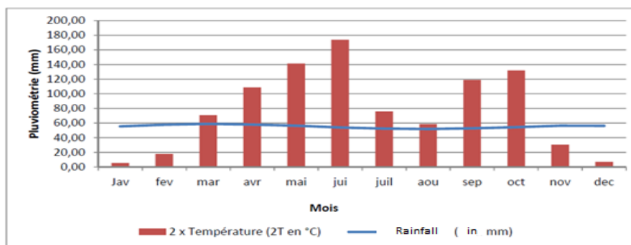
Figure n°1: Umbrothermal Diagram of the commune of Bopa (ASEENA data, 2015)
