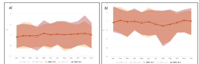
Fig 4: Projected mean temperature anomaly (°C) for 2020-2039 over the year at Tahoua
