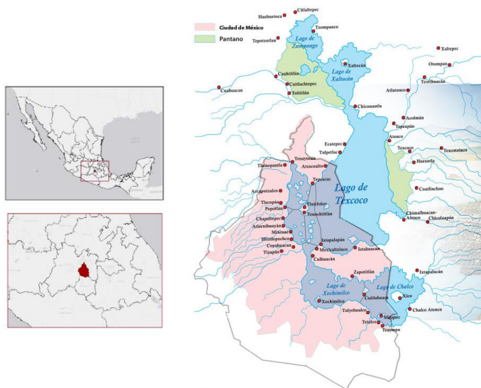
Figure 1. Extent of the Valley of Mexico and its five water bodies: Lagoon Zumpango, Lake Xaltocán, Lake Texcoco, Lake Xochimilco, and lake Chalco, (from north to south), and Mexico City location and boundaries. Source: National Autonomous University of Mexico
