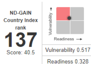
Fig. 1 Zambia ND-GAIN Index
