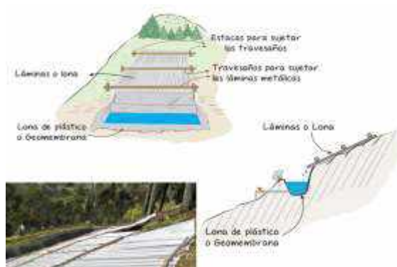
Figure 9: Water harvesting by taking advantage of existing slopes
