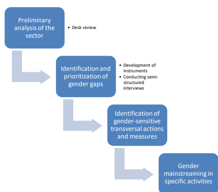
Fig. 1 Methodology
