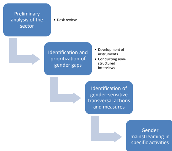
Fig. 1 Methodology
