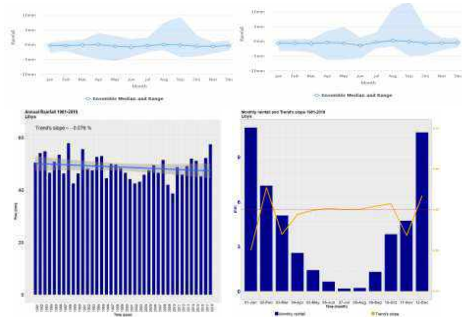
Figure 27 Projected Change in Monthly Precipitation under RCP 2.6 (Left) and RCP 8.5 (Right) in Libya between 2080 and 2099
