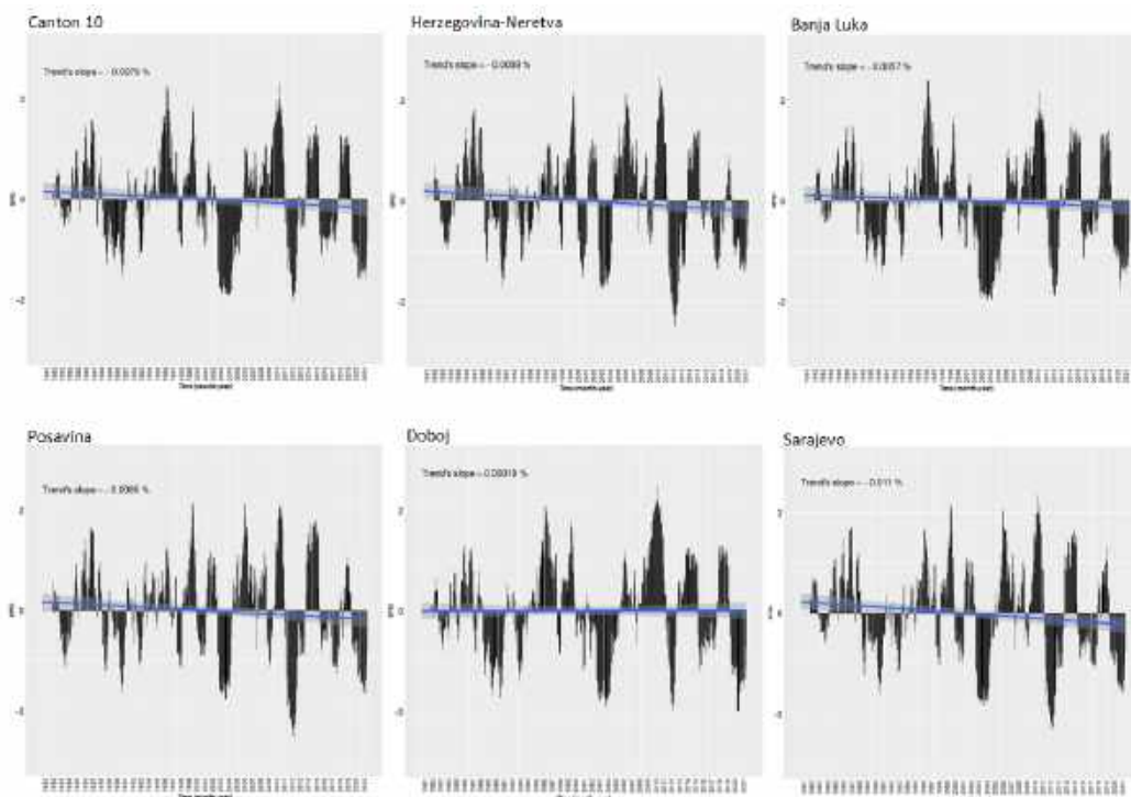
Figure 5: Monthly long term Drought index 20 (SPEI 18 months) for the Canton 10, Herzegovin-Neretva canton, Banja Luka region, Posavina canton, Dobož region and Sarajevo canton for the period 1981-2021. Source: CHIRPS, TerraClimate.
