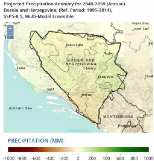
Figure 7: Projected Precipitation Anomaly for 2040-2059 in BiH compared to the reference period 1955-2014, SSP2-4.5 and SSP5-8.5, Multi-Model Ensemble. Source: CCKP.
