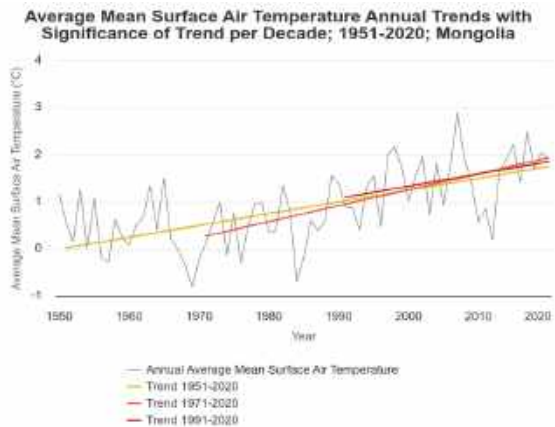
Figure 22: Annual Mean Surface Air Temperature Annual Trends with Significance of Trend per Decade; 1951-2020
