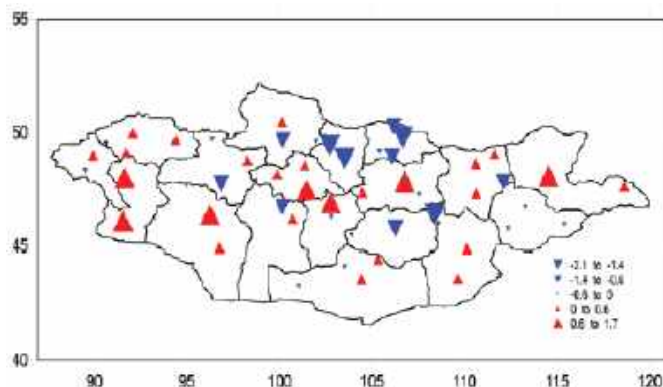
Figure 33: Change of Maximum Number of Consecutive Precipitation Days 1971-2015 (MET, 2017)
