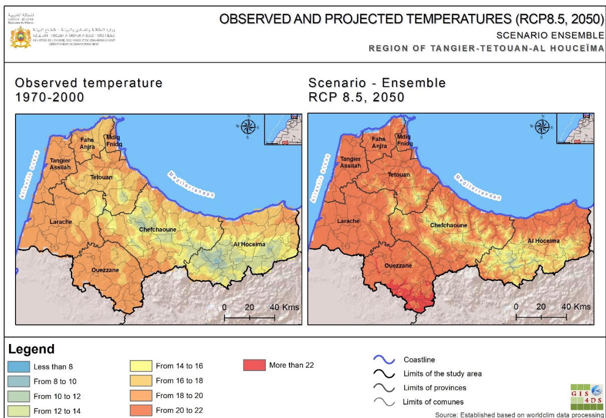
Fig 2. Observed and projected temperatures TTA to 2050 (RCP8.5)
