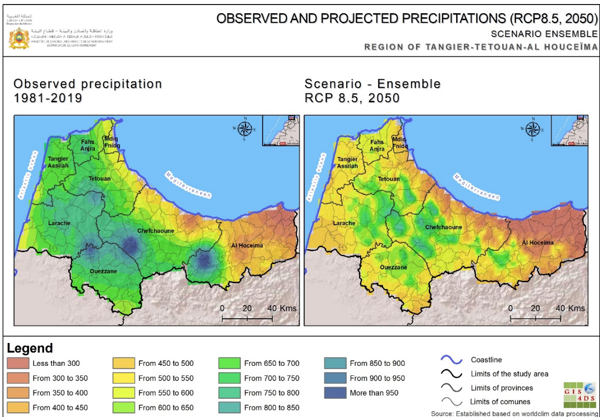
Fig 1. Observed and projected precipitation TTA in 2050
