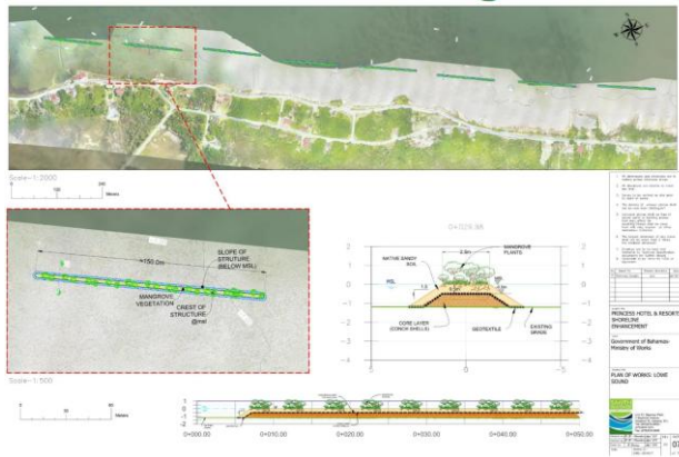
Figure 9. Sketch of approximate location and typical cross-section of the mangrove islets Source: Smith Warner International Limited, 2022
