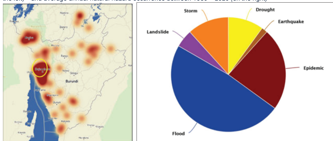
Figure 2 Climate change hazards including floods, landslides, droughts, storms and wildfires hotspots in Burundi (on the left) 14 and average annual natural hazard occurrence between 1980 – 2020 (on the right) 15
