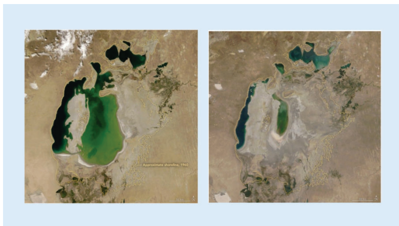
Figure 2: Aral Sea Shrinkage 2000 (left) and 2018 (right)
