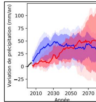
Figure 7: Average annual rainfall projections in Chad for different GHG emission scenarios, relative to the year 2000
