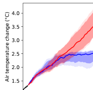
Figure 4: Air temperature projections for Chad
