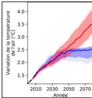
Figure 6: Air temperature projections in Chad for different GHG emission scenarios
