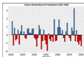
Figure 88: precipitation anomalies in the Mouhoun basin in Samendéni according to the scenarios considered.
