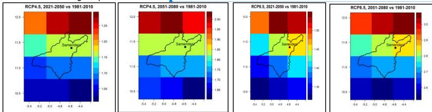
Figure 77: temperature anomalies in the Mouhoun basin in Samendéni according to the scenarios considered.
