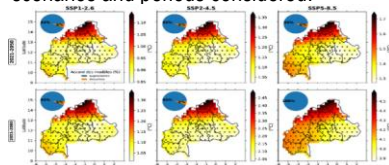
Map 12 : temperature changes in the country from 2021 to 2080.
