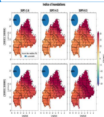
Figure 444: Flood index in BF
