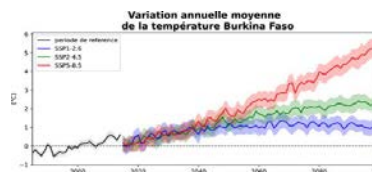
Figure 14 : average temperature variation in BF.
