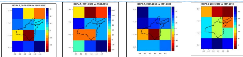
Figure 88: precipitation anomalies in the Mouhoun basin in Samendéni according to the scenarios considered.
