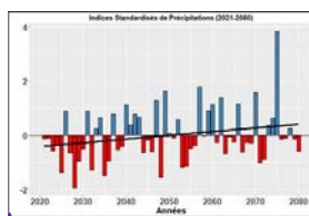
Figure 88: precipitation anomalies in the Mouhoun basin in Samendéni according to the scenarios considered.
