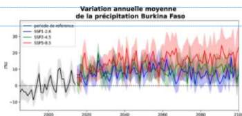
Figure 222: precipitation variation in BF
